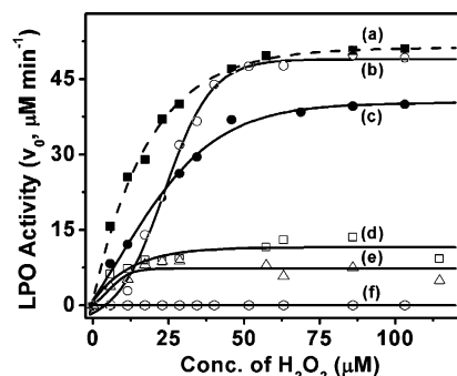
Figure 7. Plot of initial rates ( v_0 ) for the LPO-catalyzed oxidation of ABTS vs concentration of \text{H}_2\text{O}_2 . (a) Control activity, (b) 40 \mu\text{M} of 2b , (c) 40 \mu\text{M} of 8 , (d) 80 \mu\text{M} of PTU , (e) 80 \mu\text{M} of MTU , (f) 40 \mu\text{M} of MMI . Conditions: LPO: 6.5 \text{ nM} ; \text{H}_2\text{O}_2 : 22.9 \mu\text{M} .
